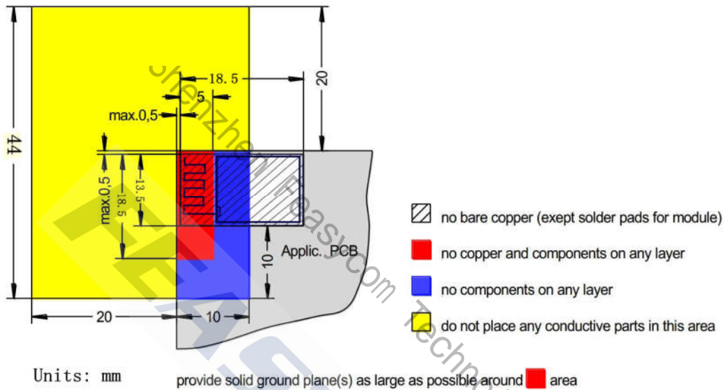
Figure 6: FSC-BT624 Restricted Area
