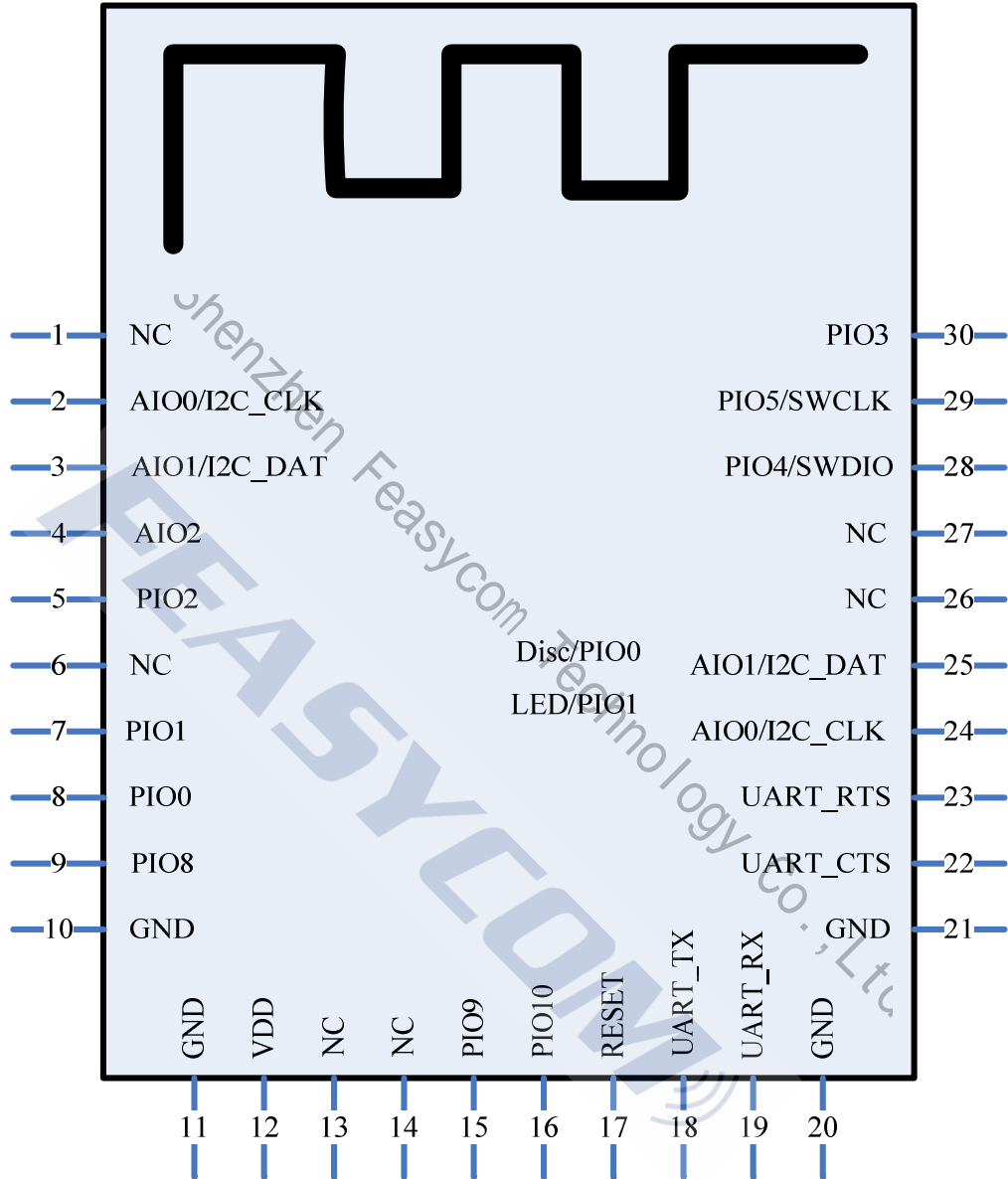
Figure2: FSC-BT624 PIN Diagram
